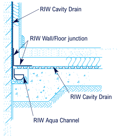
DETAIL 4 DETAIL AT WALL - FLOOR JUNCTION USING RIW AQUA CHANNEL.
