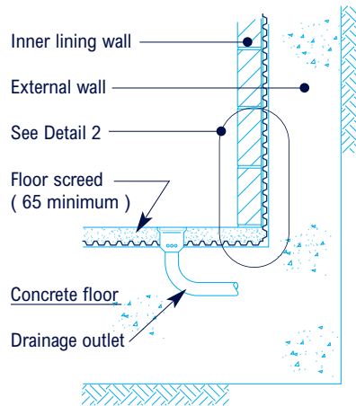
DETAIL 1 TYPICAL FLOOR / WALL DETAIL
