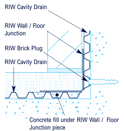
DETAIL 2 WALL - FLOOR JUNCTION
