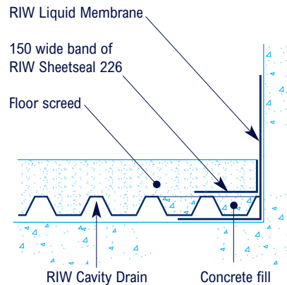
DETAIL 3 DETAIL AT COLUMNS, SERVICE, PIPES ETC .
