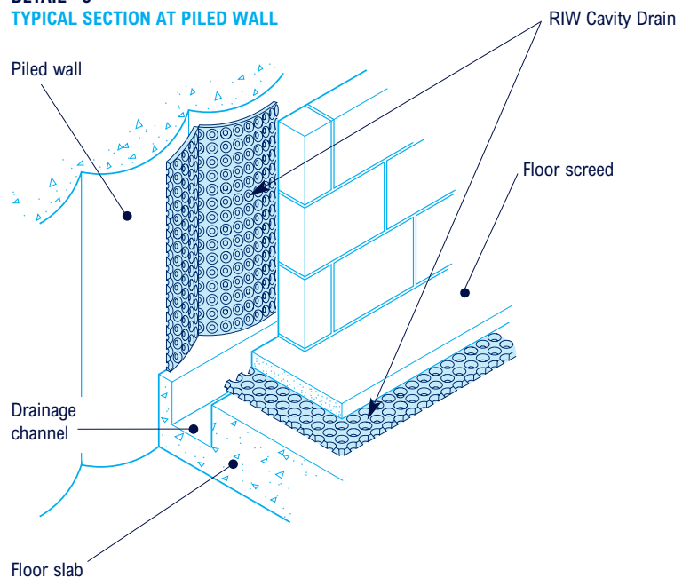
DETAIL 5 TYPICAL SECTION AT PILED WALL
