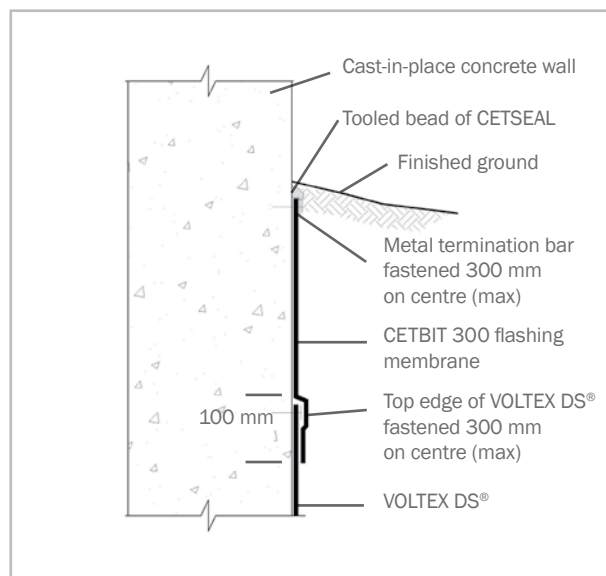
Ground Termination
